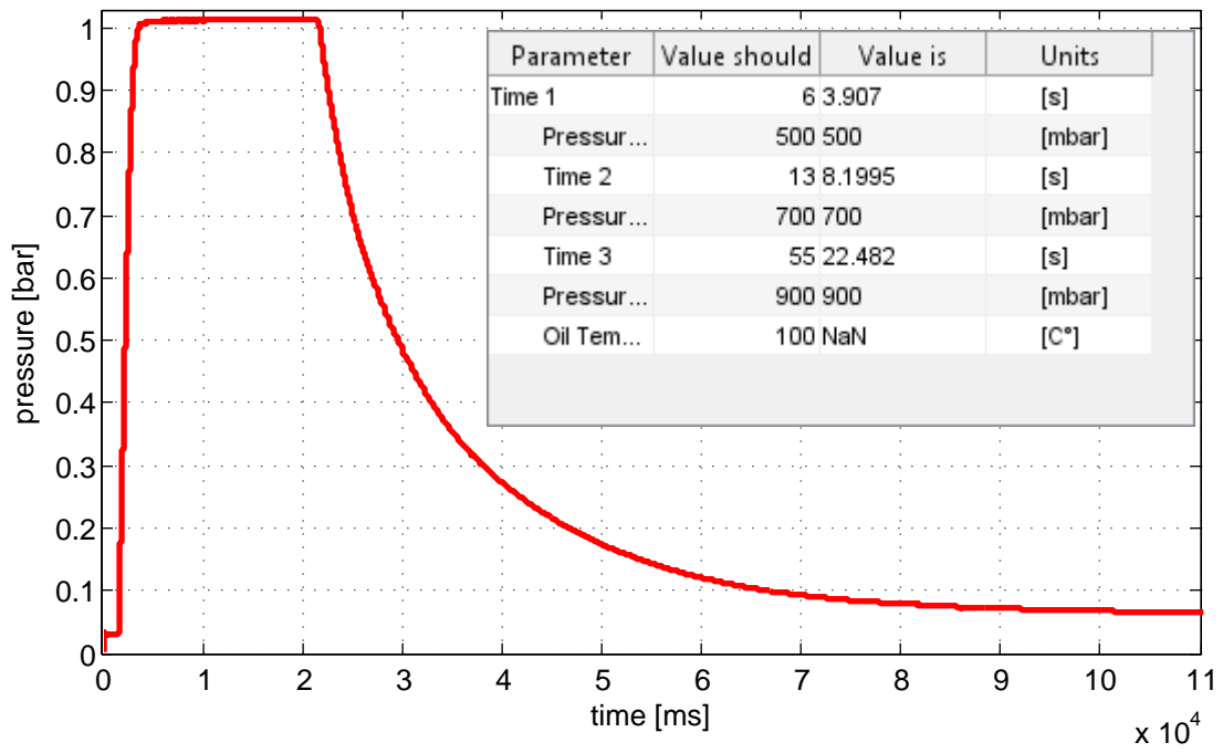
Performance curve
