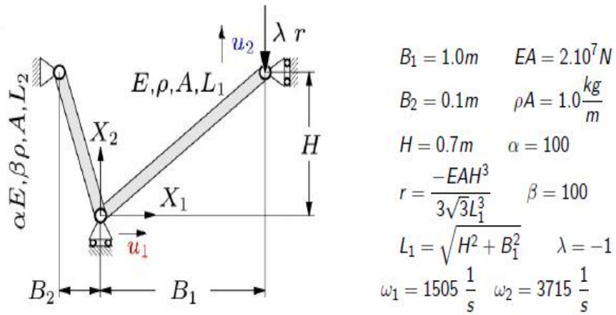
Fig. 7.5: Two linear trusses model (Gleim [28])
