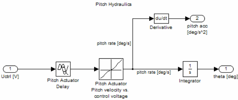
Figure 96 Model of the pitch system implemented in Matlab/ Simulink
