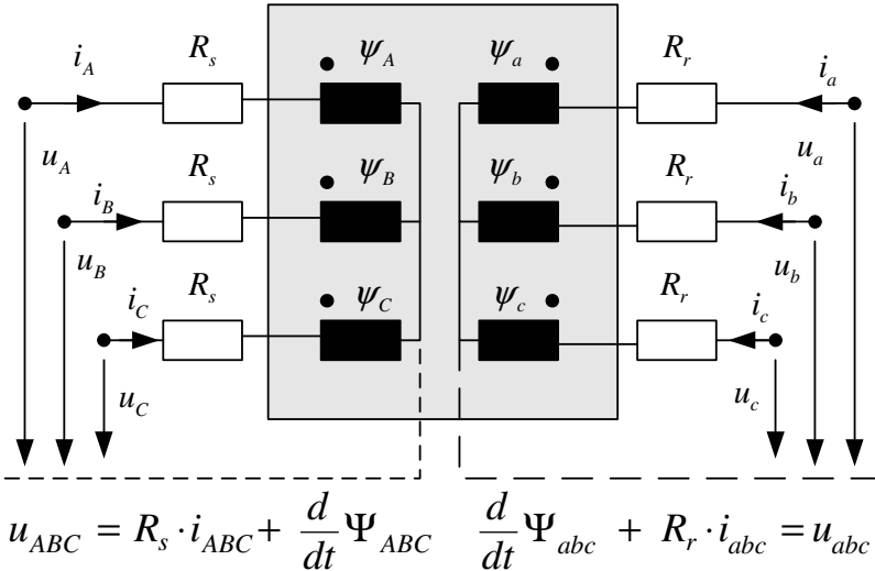
Figure 45 Three phase equivalent ABC/abc circuit diagram of a doubly fed induction machine
