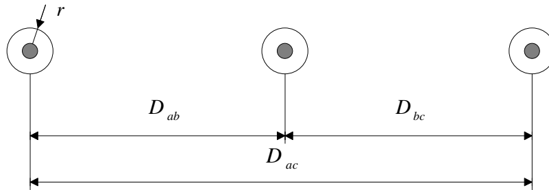
Figure 82 Inductance of a three phase overhead line
