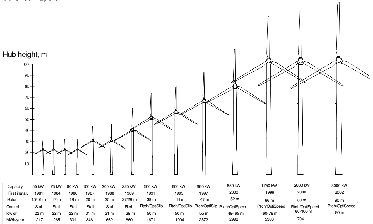
Figure 227 Vestas Type Development
